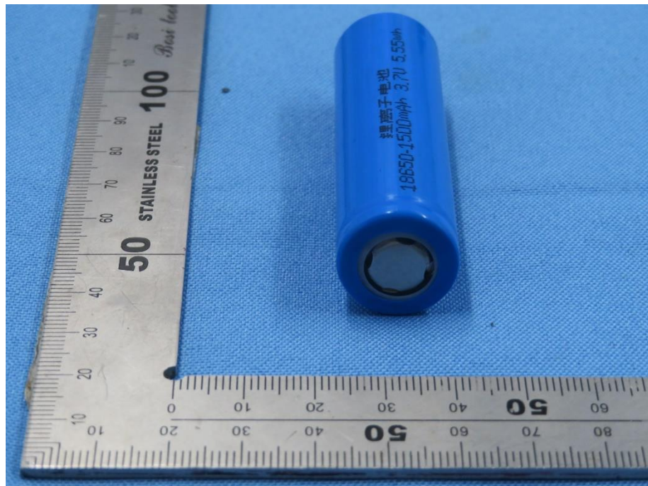
Picture 2. Side view of cell (IMR18650-1500mAh)
