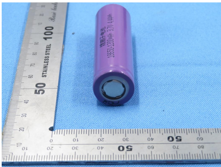
Picture 4. Side view of cell (IMR18650-1200mAh)
