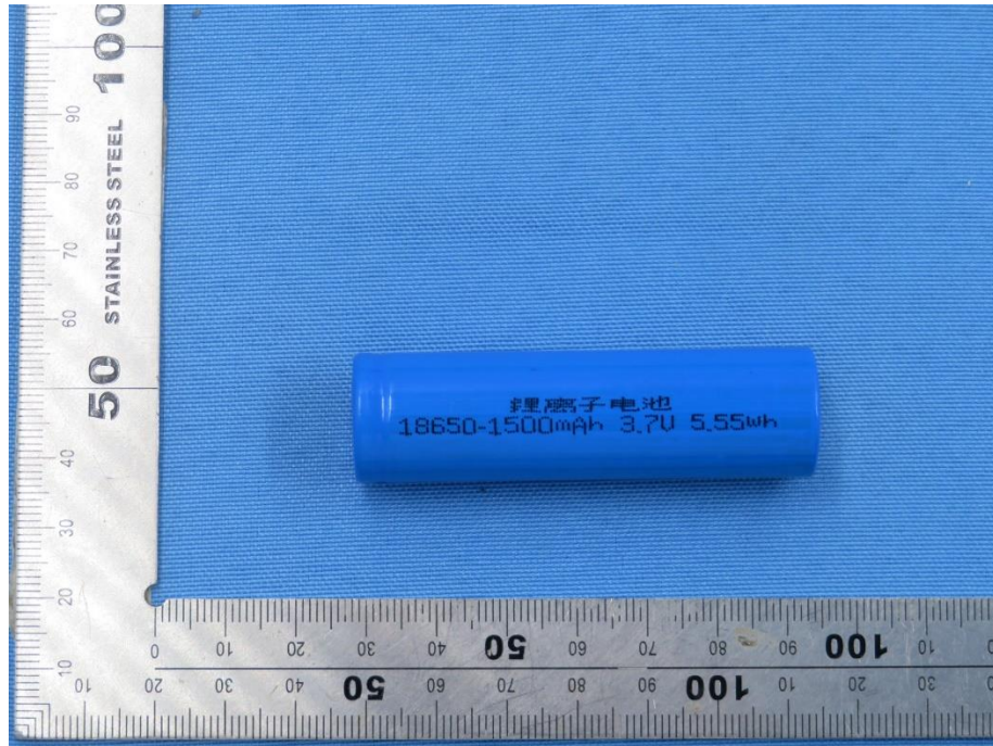
Picture 1. Main view of cell (IMR18650-1500mAh)
