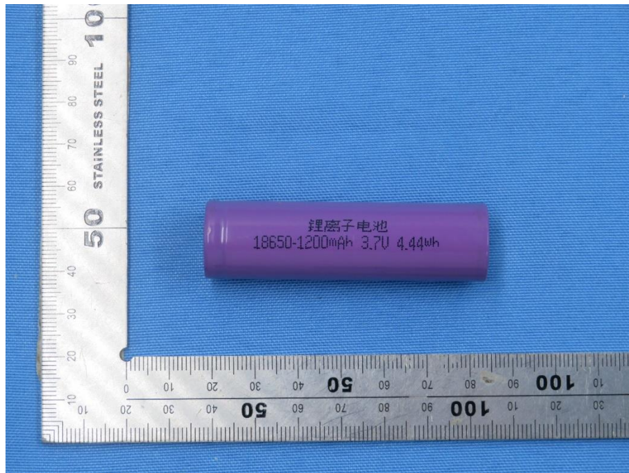
Picture 3. Main view of cell (IMR18650-1200mAh)
