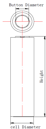
Cell 2 (IMR18650-1200mAh)
